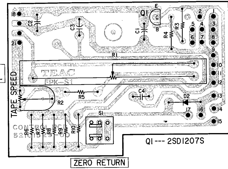
CONTROL PCB ASS'Y
