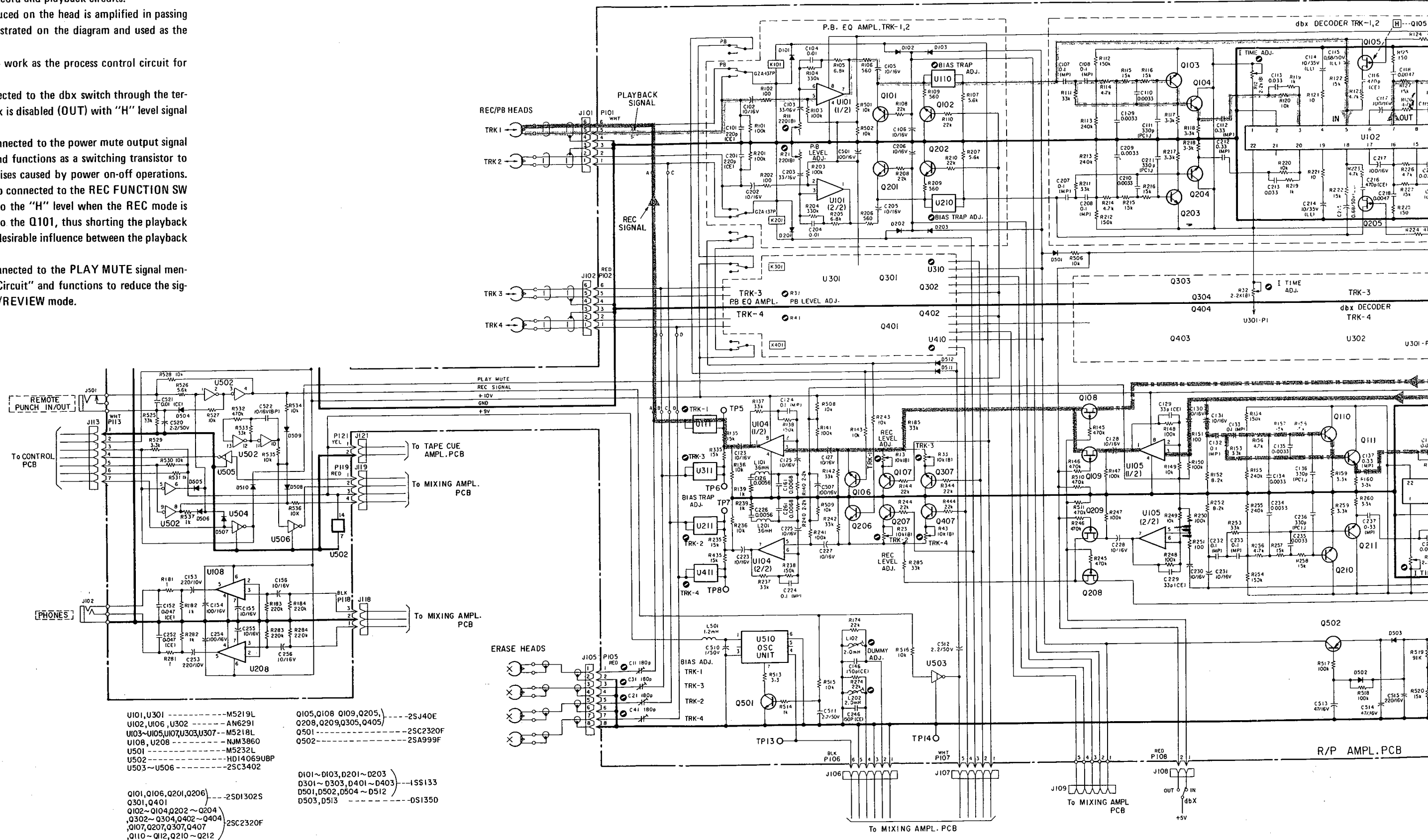
Fig. 3-6 Record & playback circuit
