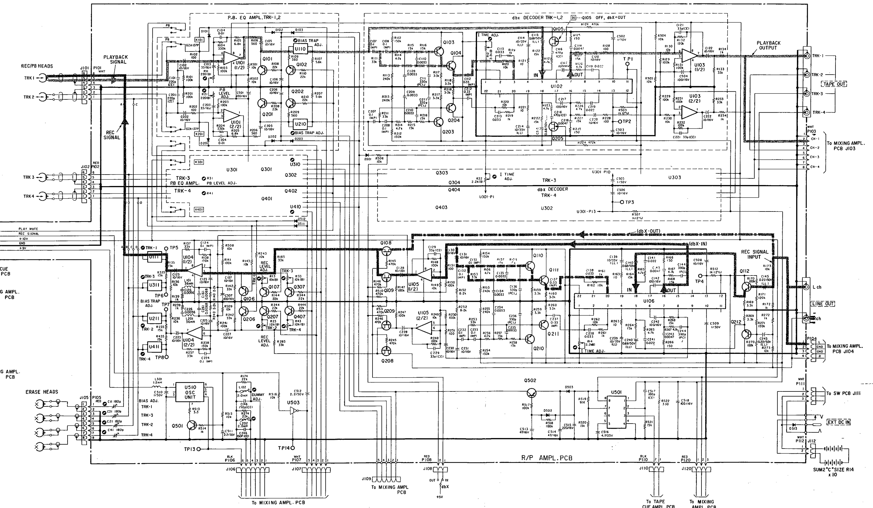
Fig. 3-6 Record & playback circuit
