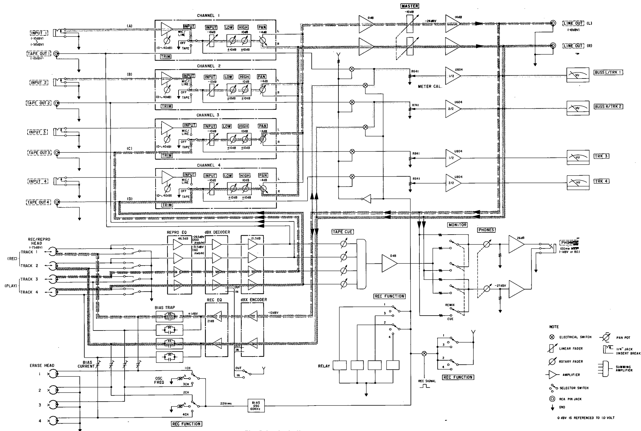
Fig. 3-1 Block diagram
