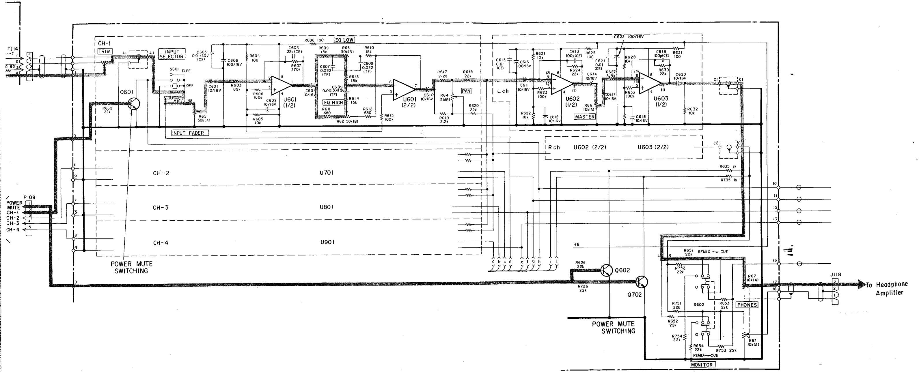
Fig. 3-5 Mixer amplifier circuit
